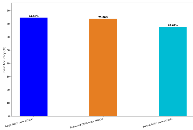
Figure 6. Final clean baseline accuracies comparing AEGIS against Sybil-centric (FoolsGold) and meta-aggregation (Bulyan) defenses.
